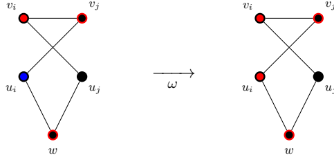
Fig. 2: Schematic form of the argument for the PR inference. With c = \text{Red} and c' = \text{Blue} , the above diagram shows the transformation we can apply to a solution to obtain another valid solution. A vertex colored black on the inside means that it does not have the outer color, i.e. w has some color other than red. Unit propagation implies that v_j is not colored red.
